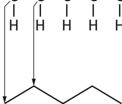
pentane
